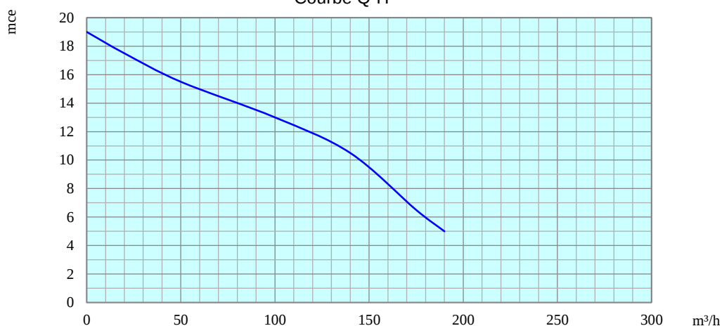
Courbe Q-H
